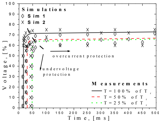
Fig. 4. Influence of different torque values on sensitivity of PWM drive to symmetrical three-phase voltage sags.
