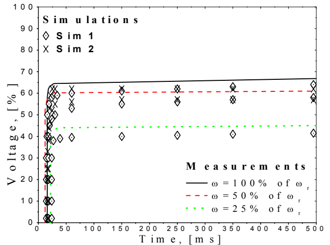
Fig. 6. Influence of different motor speeds on sensitivity of PWM drive to symmetrical two-phase voltage sags with rated voltage in unsagged phase.
