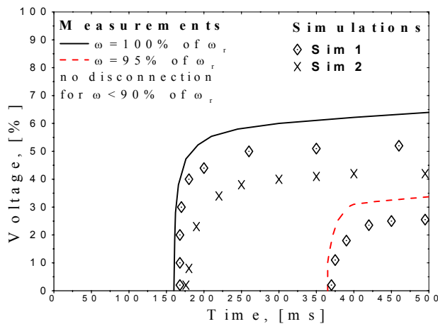
Fig. 7. Influence of different motor speeds on sensitivity of PWM drive to single-phase voltage sags with rated voltage in two unsagged phases.
