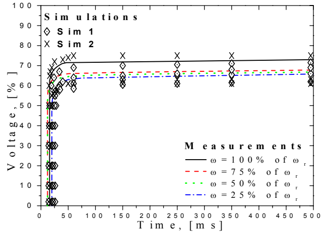
Fig. 5. Influence of different motor speeds on sensitivity of PWM drive to symmetrical three-phase voltage sags.
