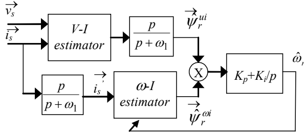
Fig.5. Modified MRAS speed estimation scheme
