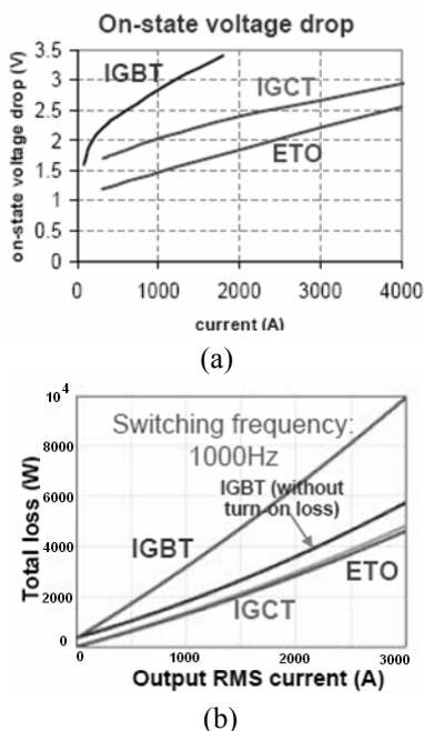
Fig. 10 Comparisons of the device's (a) on-state voltage drop, (b) total losses in a PWM voltage source converter with sinusoid output [19]
