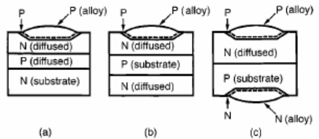
Fig. 6. Schematic cross sections [10] of three forms of Si p-n-p-n switches made at Bell Telephone Laboratories (BTL) in 1955. The switch shown in (b) became the Si controlled rectifier (SCR) at GE in 1957.
