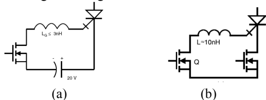
Fig. 9 Circuit representation: (a) IGCT, (b) ETO [18]
