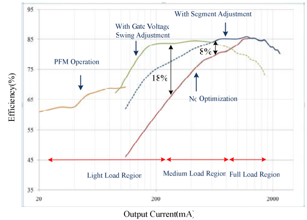
Fig.4. Power processing efficiency comparison of a 2A dc-dc buck converter.
