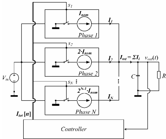
Fig.7. Multi-phase CPM converter with logarithmic current sharing.
