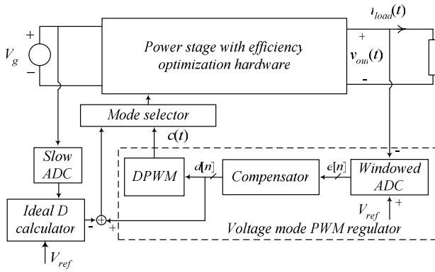
Fig.5. Duty ratio based optimization system.
