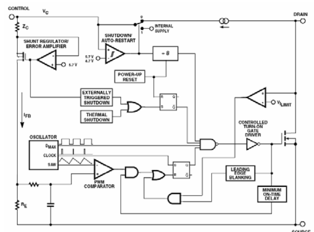
Fig. 1. Simplified internal structure of TOPSwitch
