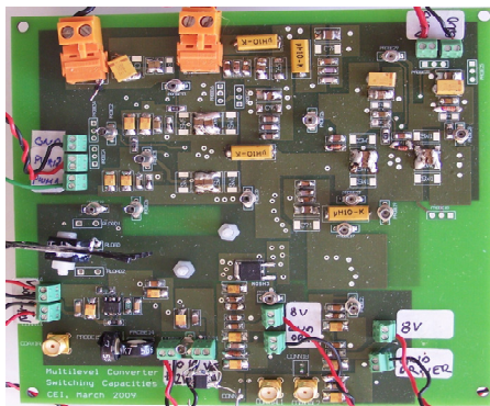
Fig. 9. Photograph of implemented multilevel converter, architecture one
