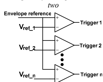
Fig. 8. Comparator logic that is used to control on/off states for each cell/switch of the multilevel converter/analog multiplexer
