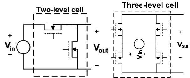
Fig. 4. Voltage cells that could be used as a solution to implement a multilevel converter
