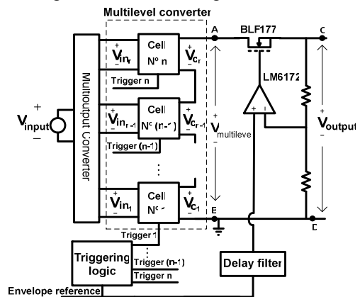
Fig. 7. Block diagram of the implemented architecture two
