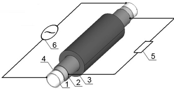
Fig. 1. Idea of linear transformer (elementary) 1-primary winding; 2-secondary winding; 3-ferrite core; 4-insulation; 5-load; 6-voltage supply
