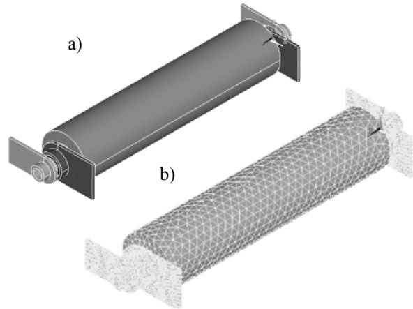
Fig. 4. a) volumes of elementary transformer of 50 mm of length; b) mesh volumes
