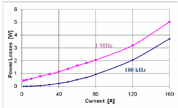
Fig. 13. Overall power losses in leads and interconnections (for input voltage of 100 V_{max} ) of experimental transformer; (4 leads, 12 interconnections)
