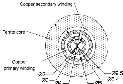
Fig. 2. Cross-section of linear transformer depicted in Fig. 1 and analyzed in this paper
