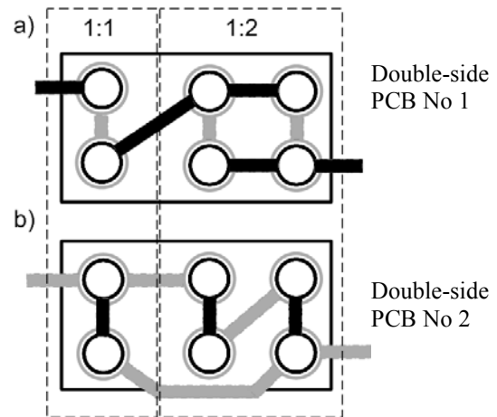
Fig. 17. Method of connection the n-modules a) front side; b) back side
