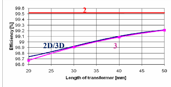
Fig. 6. Total efficiency of elementary transformer
