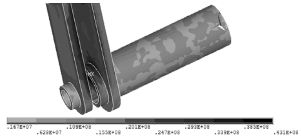
Fig. 7. Current density in interconnection.
