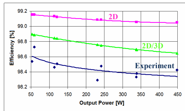
Fig. 14. Efficiency of experimental transformer
