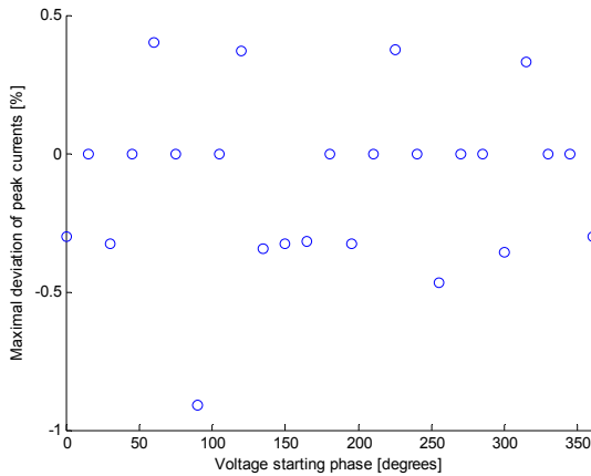
Fig. 7. Maximal deviations of inductors peak currents among repetitions
