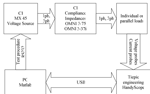
Fig. 1. Schematic diagram of the laboratory setup
