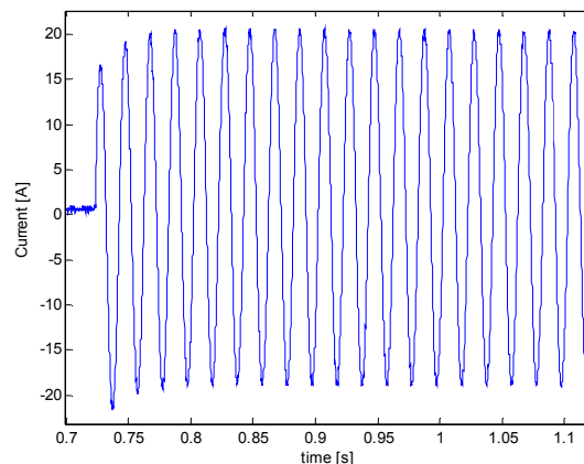
Fig. 4. Inrush current sample – 50 mH inductor
