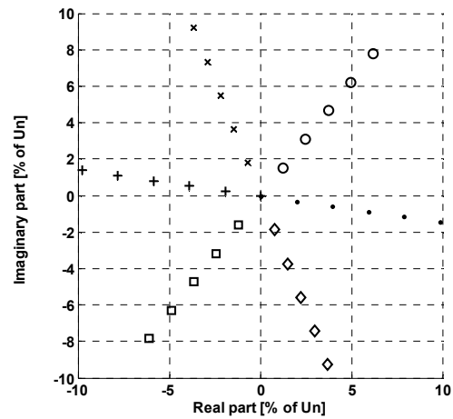
Fig. 11. Voltage values used in the test – 5 th harmonic
