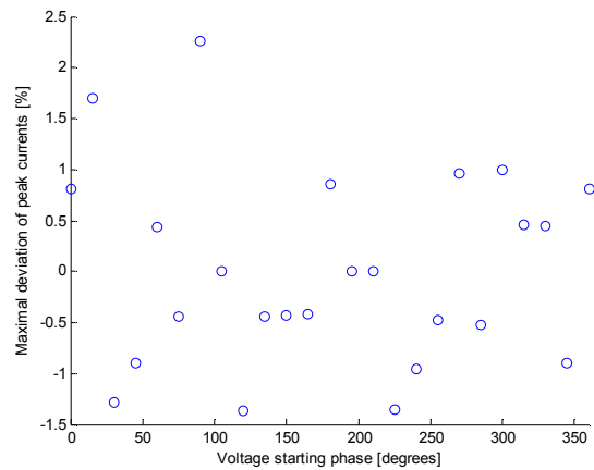
Fig. 10. Maximal deviations of vacuum cleaners peak currents among repetitions
