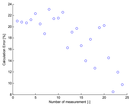
Fig. 15. Relative calculation error – ES lamp, 5 th harm.
