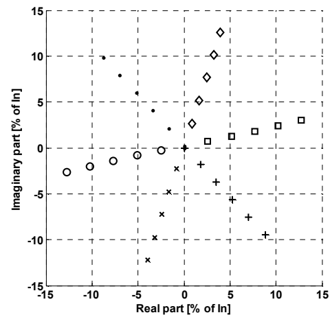
Fig. 12. Measured 5 th harmonic current – Fan
