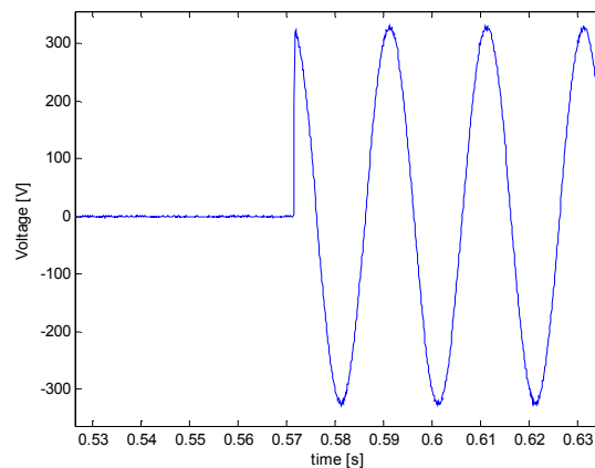
Fig. 3. Sample of the measured starting voltage
