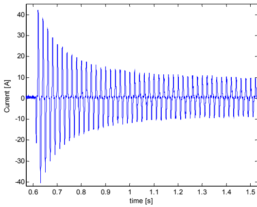
Fig. 5. Inrush current sample – Vacuum cleaner
