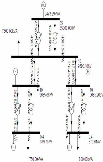
Fig. 6 Single-pole scheme model observed distribution system before the installation of filters
