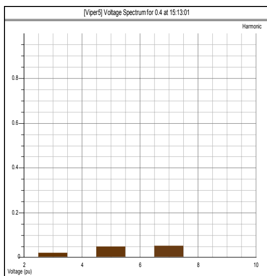
Fig. 9 Harmonic voltage spectrum of models before the installation of filters
