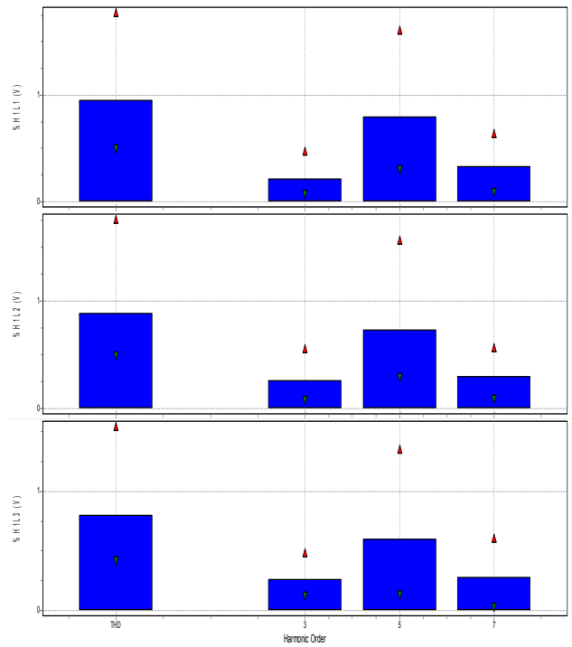
Fig. 2 THDU and voltage harmonics- HDU_3 , HDU_5 , HDU_7 (Line 1-top, Line 2-middle, Line 3-bottom)
