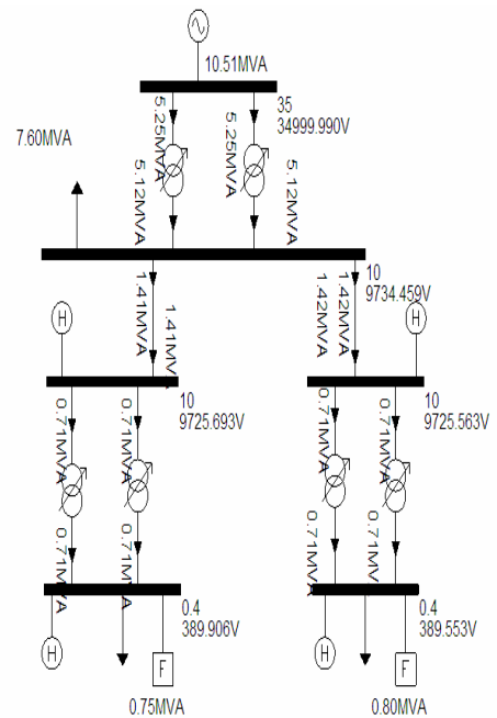
Fig. 8 Single-pole scheme model observed distribution system after the installation of filters
