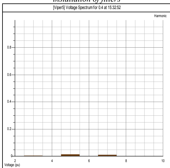
Fig. 10 Harmonic voltage spectrum of models after the installation of filters
