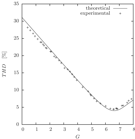
Fig. 6. Experimental results, THD(G) , with filter.
