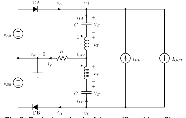
Fig. 3. Equivalent circuit of the rectifier without filter.
