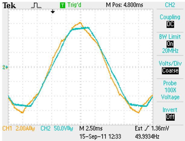
Fig. 9. Waveforms of v_1 and i_1 at I_{OUT} = 5 A and THD_{min} , without filter.
